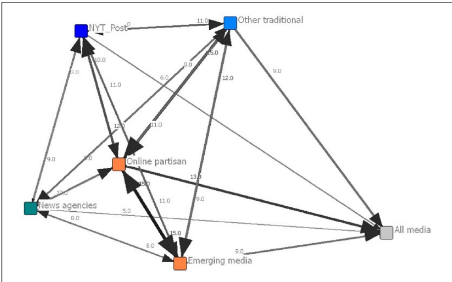
Figure 1. Directed Granger causality graph.
